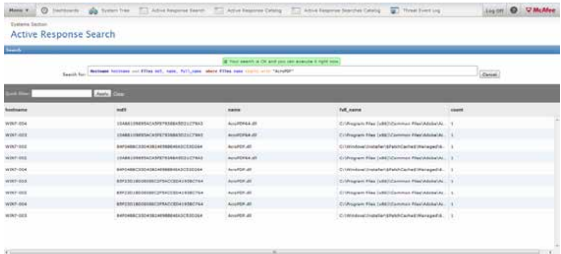
Figure 1. McAfee Active Response search user interface.
